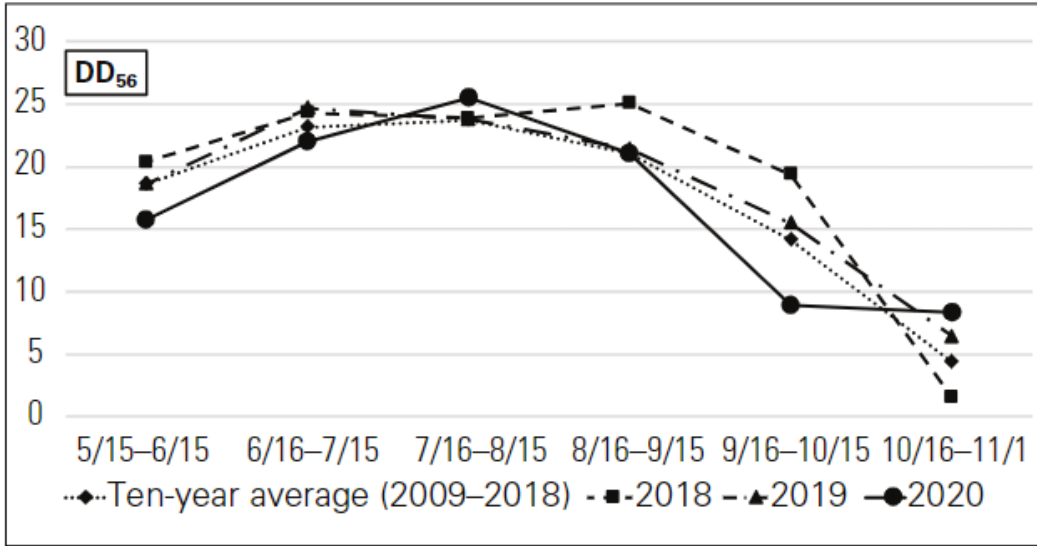
Figure 3-2. Heat Unit Accumulation (DD 56 ) at Lewiston-Woodville. Source: David Jordan
